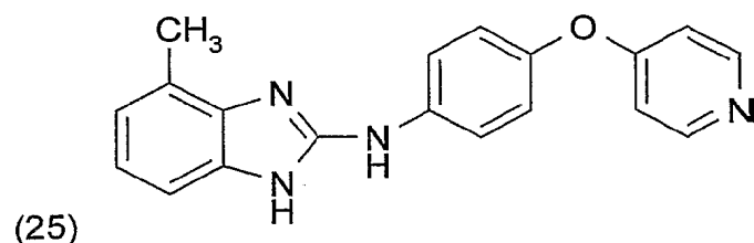
(4-Methyl-1H-benzimidazol-2-yl)-[4-(pyridin-4-yloxy)-phenyl]-amin
